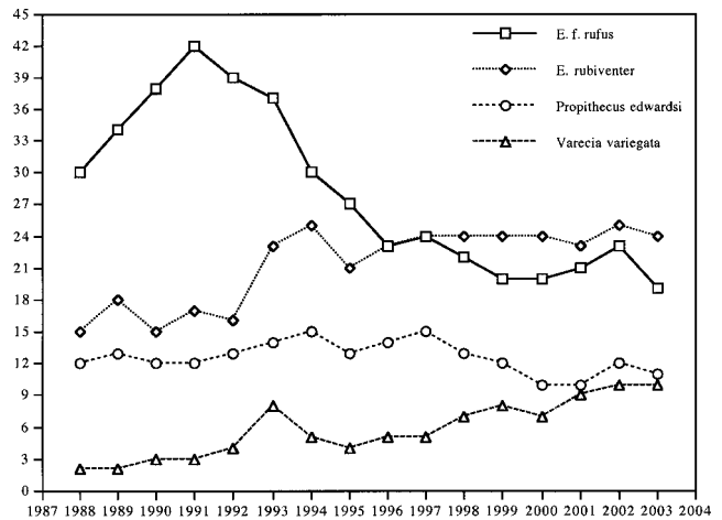
Fig. 7. Population densities (individuals per square kilometer) for frugivorous species at Vatoharanana from July 1988 to August 2003.
