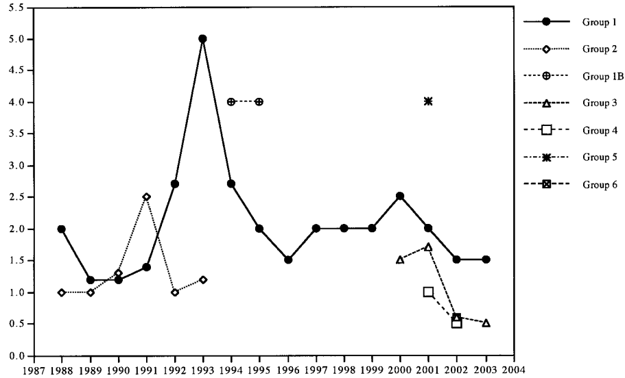
Fig. 2. Adult sex ratio in groups from July 1988 to August 2003.
