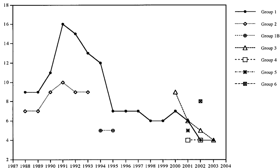
Fig. 1. Mean group size changes from July 1988 to August 2003.
