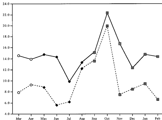
Fig. 4. The percentage of trees with fruit across reproductive and nonreproductive periods for 1988–1993 (solid line) and 1994–2003 (dashed line). Circles = nonreproductive months, diamonds = mating and gestation, squares = birth and lactation.
