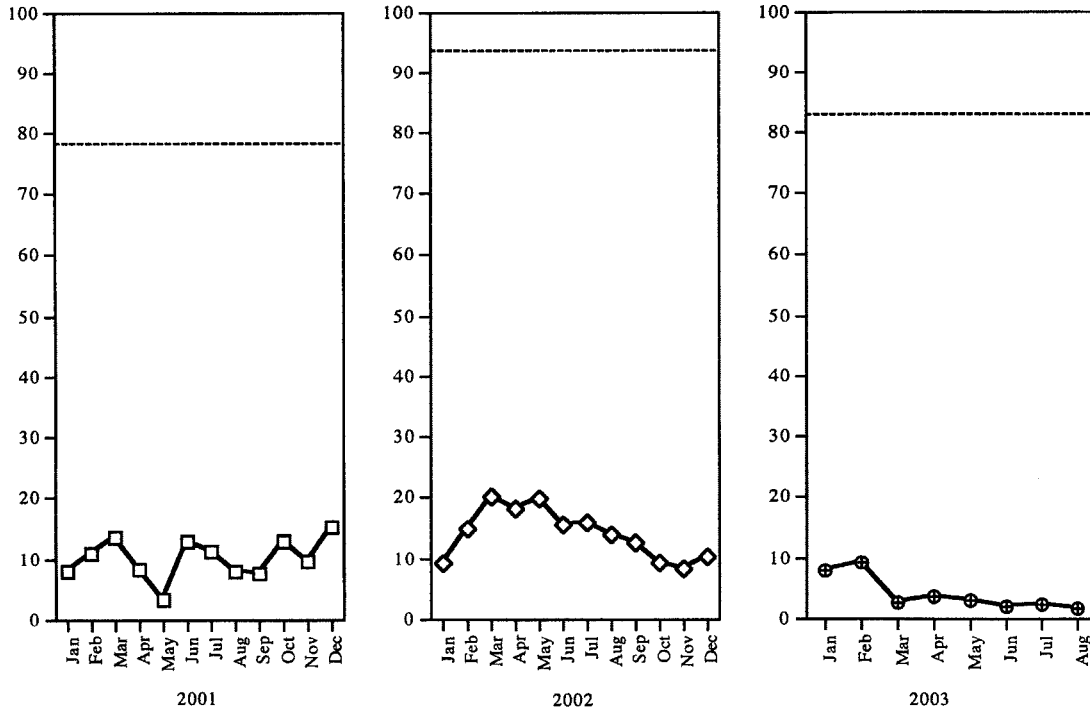
Fig. 5. The percentage of trees with fruit from January 2001 to August 2003. The dashed line across the top indicates the average amount of fruit consumption for each year. The number of trees sampled each year was 2001 = 409, 2002 = 407, and 2003 = 387.
