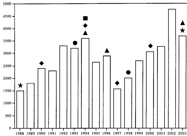
Fig. 6. Rainfall data from July 1988 to August 2003. The symbols above the bars indicate tropical storms and cyclones. Circles indicate tropical storms, stars indicate category 1 cyclones, triangles indicate category 2 cyclones, diamonds indicate category 4 cyclones, and squares indicate category 5 cyclones.
